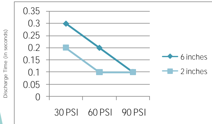
Offset voltage and discharge time per ESDA standard S3.1 using a charged plate monitor with a 20pF, 6" x 6" plate. Typical results. 1000 to 100 volts.
